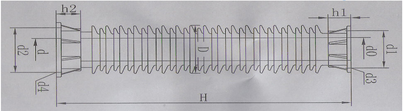
72.5KV-126KV SF 6 Circuit Breaker Post Hollow Insulators (Table 1)
